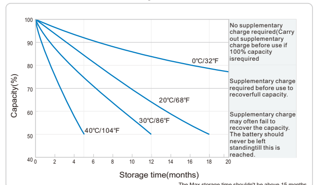
Self-discharge Characteristic
